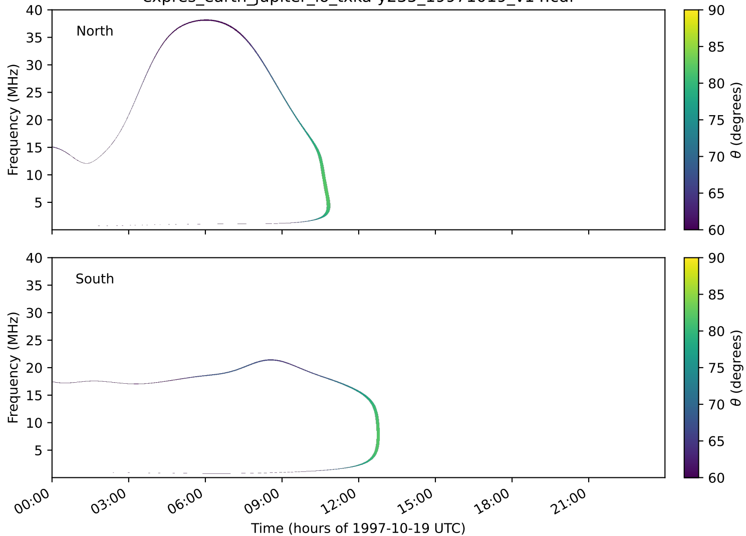
expres_earth_jupiter_io_txka-y235_19971019_v14.cdf
