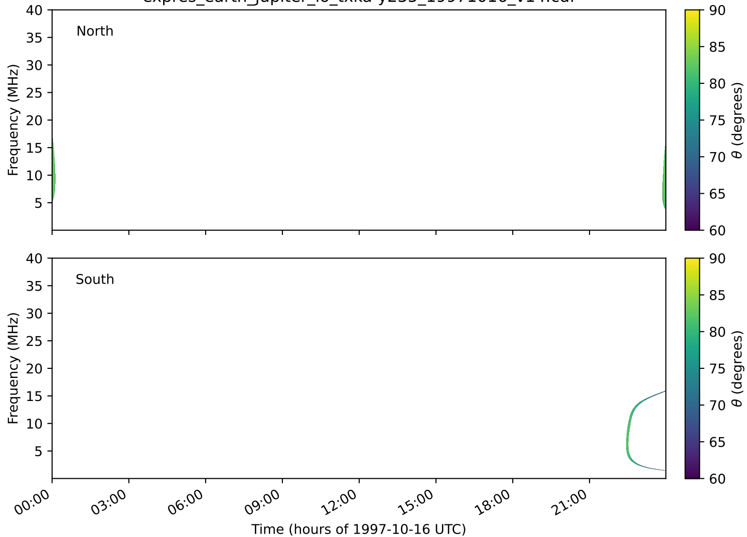
expres_earth_jupiter_io_txka-y235_19971016_v14.cdf
