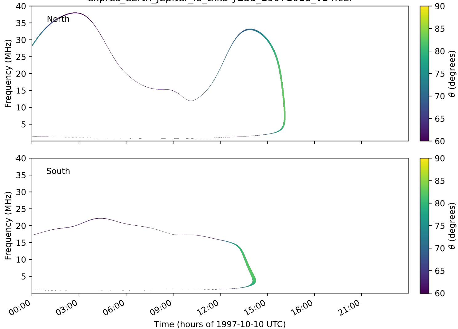
expres_earth_jupiter_io_txka-y235_19971010_v14.cdf
