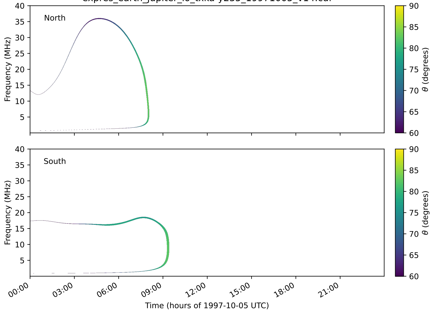
expres_earth_jupiter_io_txka-y235_19971005_v14.cdf
