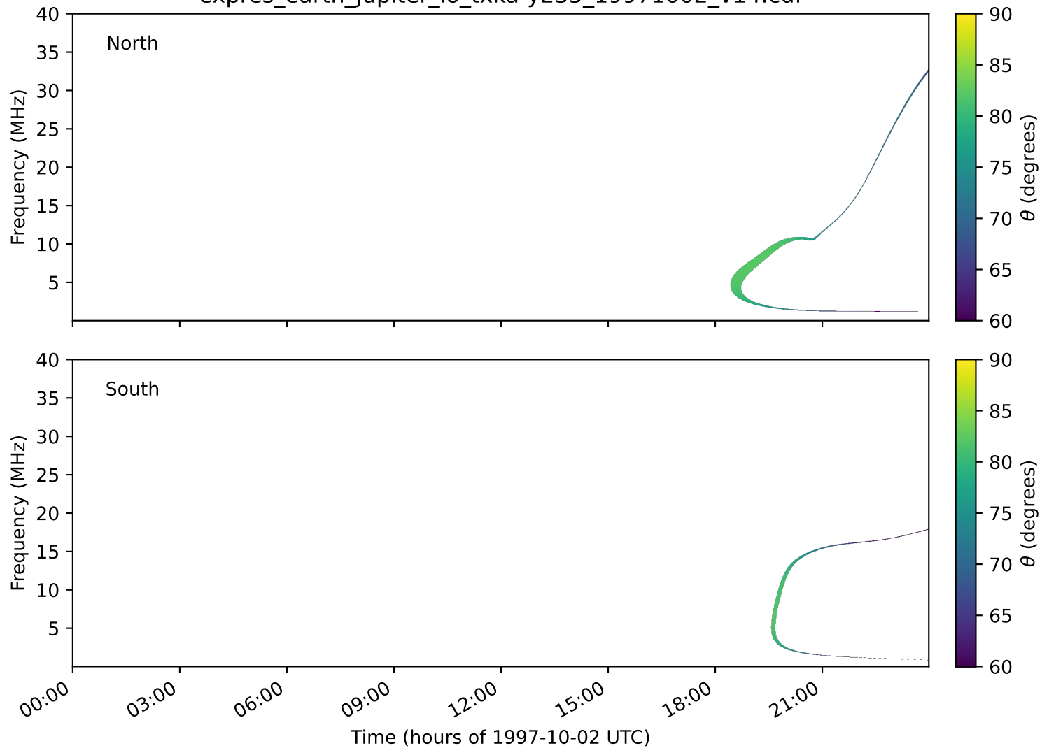
expres_earth_jupiter_io_txka-y235_19971002_v14.cdf
