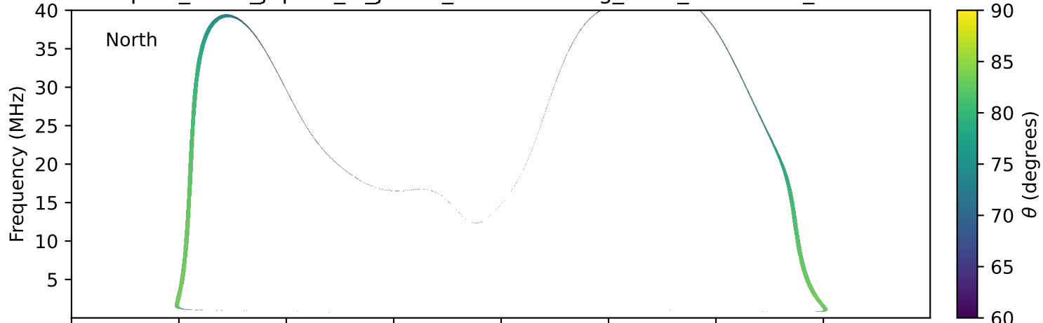
expres_earth_jupiter_io_jrm33_lossc-wid1deg_3kev_19971031_v11.cdf
