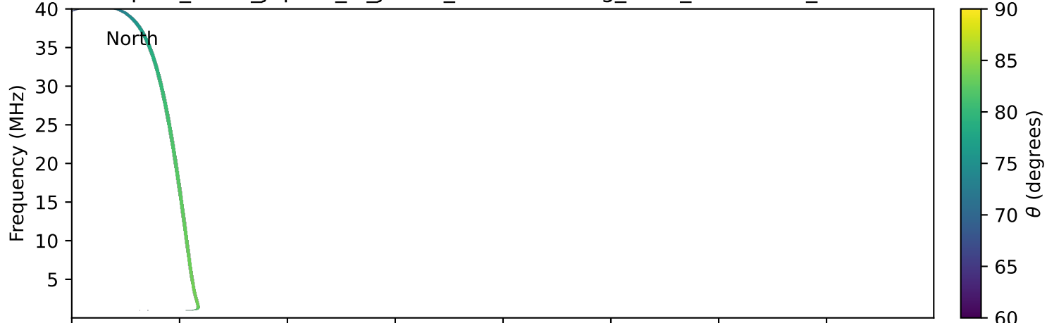
expres_earth_jupiter_io_jrm33_lossc-wid1deg_3kev_19971030_v11.cdf
