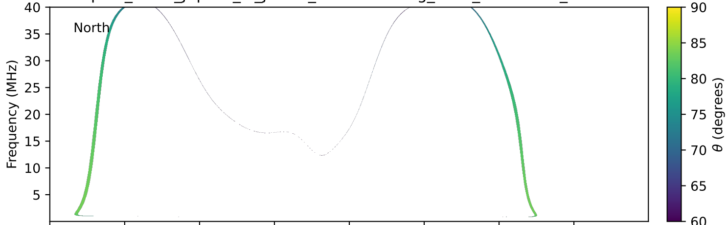
expres_earth_jupiter_io_jrm33_lossc-wid1deg_3kev_19971024_v11.cdf
