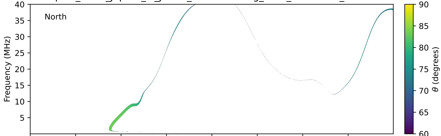
expres_earth_jupiter_io_jrm33_lossc-wid1deg_3kev_19971022_v11.cdf
