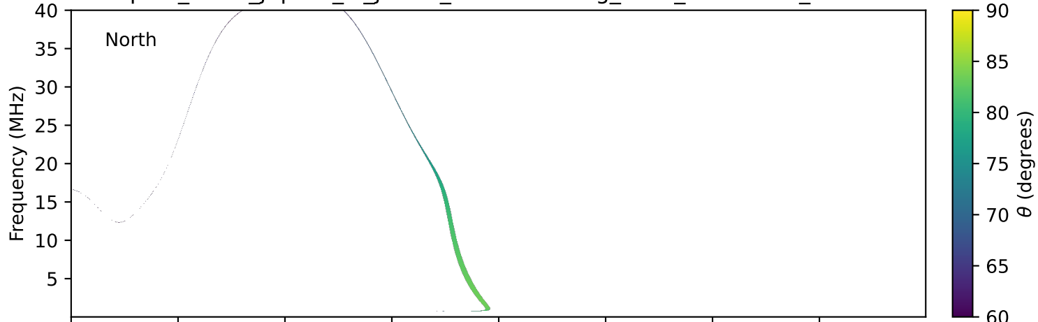
expres_earth_jupiter_io_jrm33_lossc-wid1deg_3kev_19971019_v11.cdf
