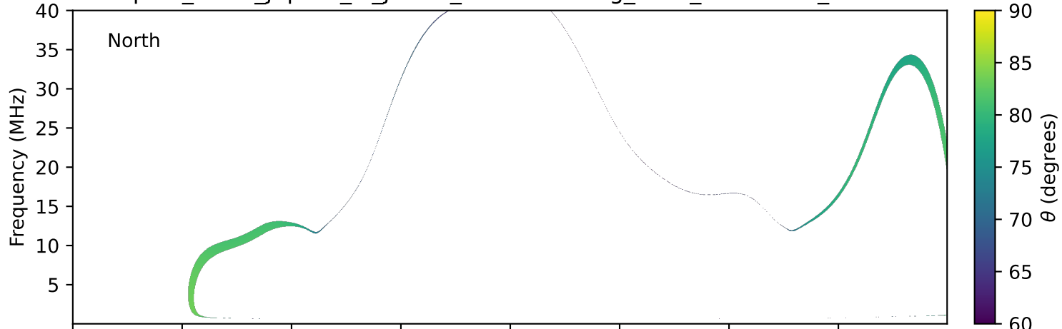
expres_earth_jupiter_io_jrm33_lossc-wid1deg_3kev_19971015_v11.cdf
