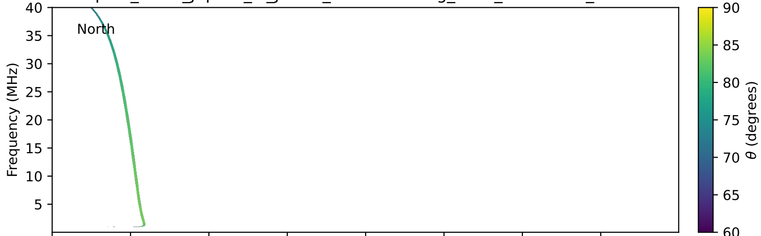
expres_earth_jupiter_io_jrm09_lossc-wid1deg_3kev_19971030_v11.cdf
