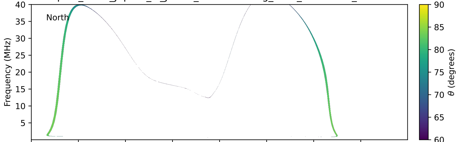
expres_earth_jupiter_io_jrm09_lossc-wid1deg_3kev_19971024_v11.cdf
