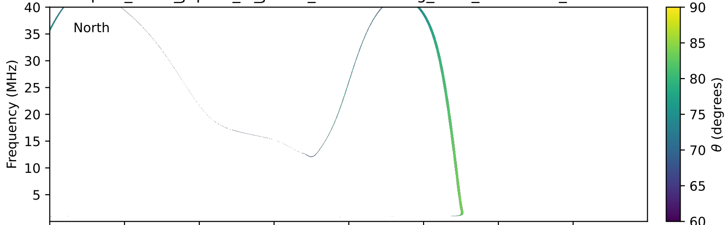
expres_earth_jupiter_io_jrm09_lossc-wid1deg_3kev_19971010_v11.cdf
