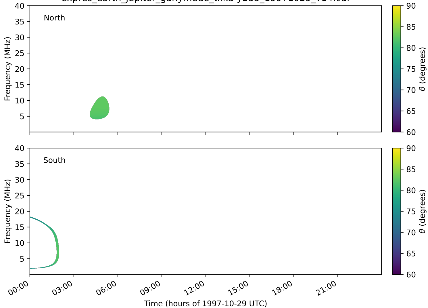
expres_earth_jupiter_ganymede_txka-y235_19971029_v14.cdf
