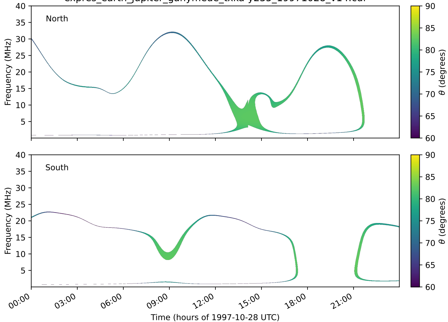
expres_earth_jupiter_ganymede_txka-y235_19971028_v14.cdf
