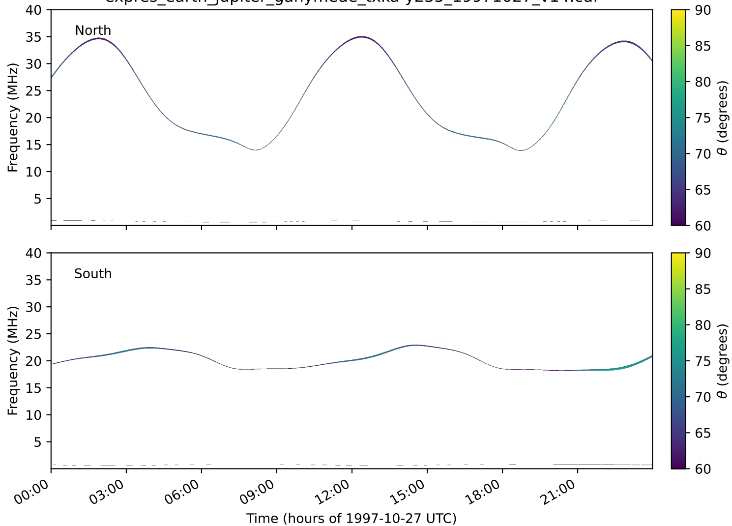
expres_earth_jupiter_ganymede_txka-y235_19971027_v14.cdf
