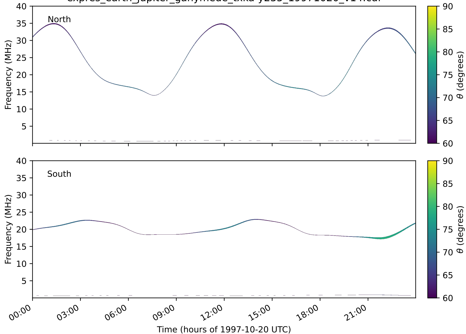
expres_earth_jupiter_ganymede_txka-y235_19971020_v14.cdf
