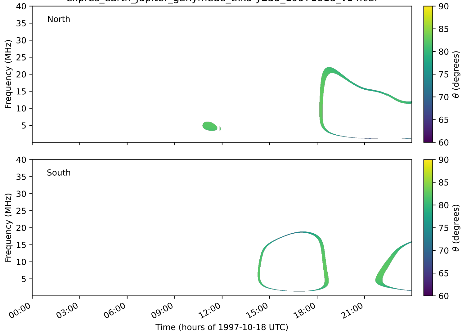
expres_earth_jupiter_ganymede_txka-y235_19971018_v14.cdf
