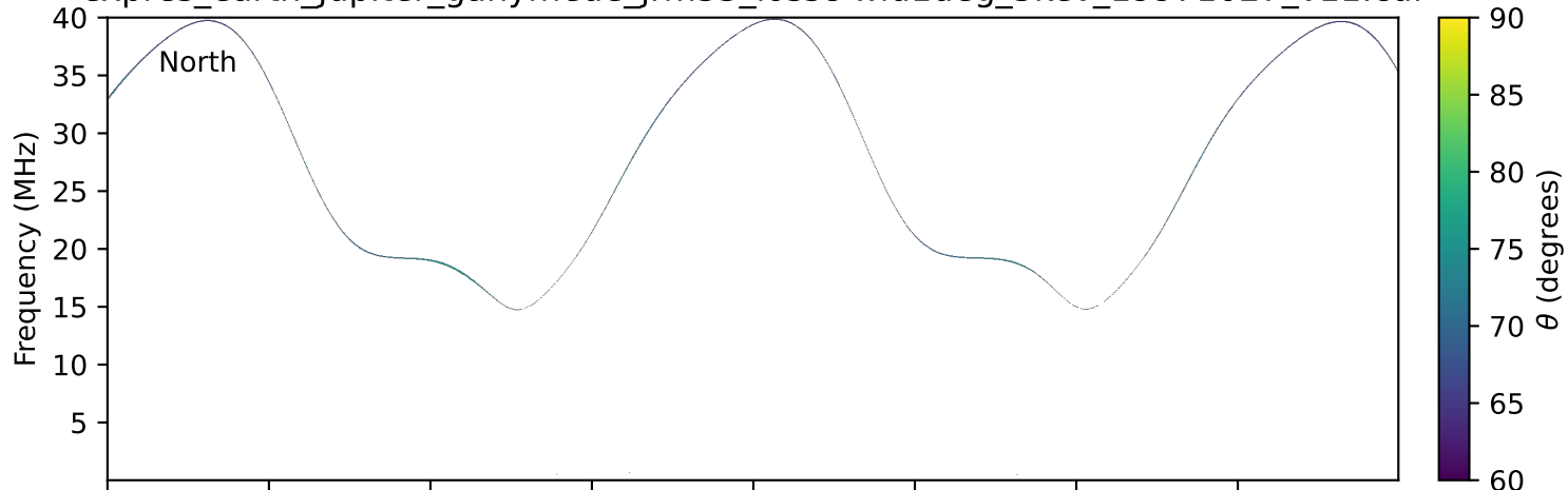
expres_earth_jupiter_ganymede_jrm33_lossc-wid1deg_3kev_19971027_v11.cdf
