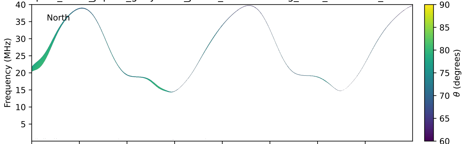
expres_earth_jupiter_ganymede_jrm33_lossc-wid1deg_3kev_19971005_v11.cdf
