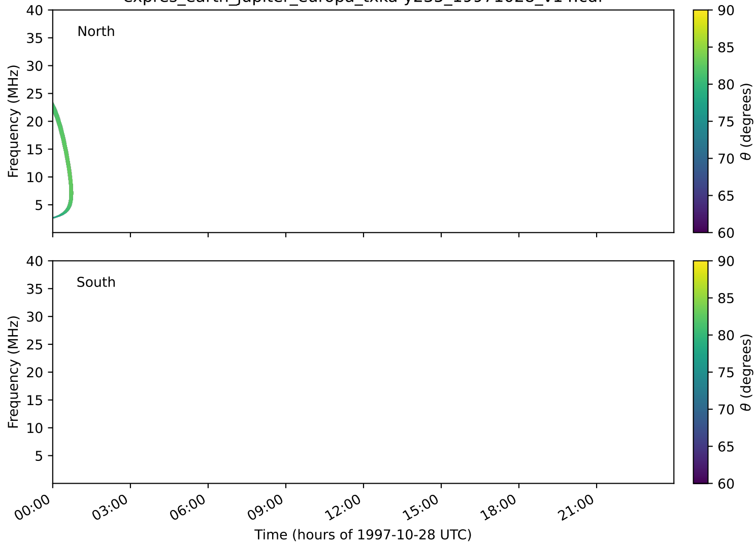
expres_earth_jupiter_europa_txka-y235_19971028_v14.cdf
