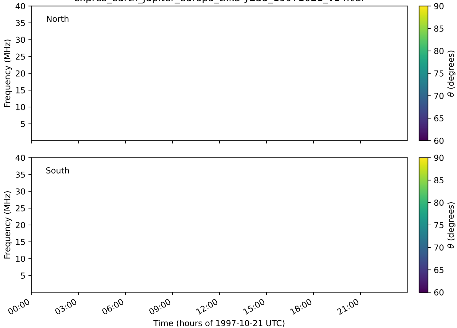
expres_earth_jupiter_europa_txka-y235_19971021_v14.cdf
