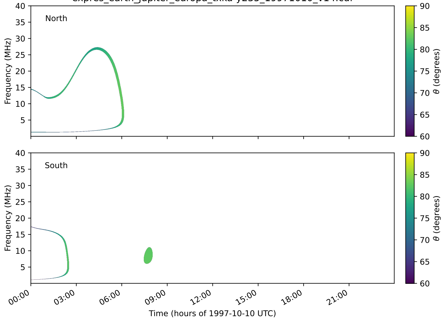
expres_earth_jupiter_europa_txka-y235_19971010_v14.cdf
