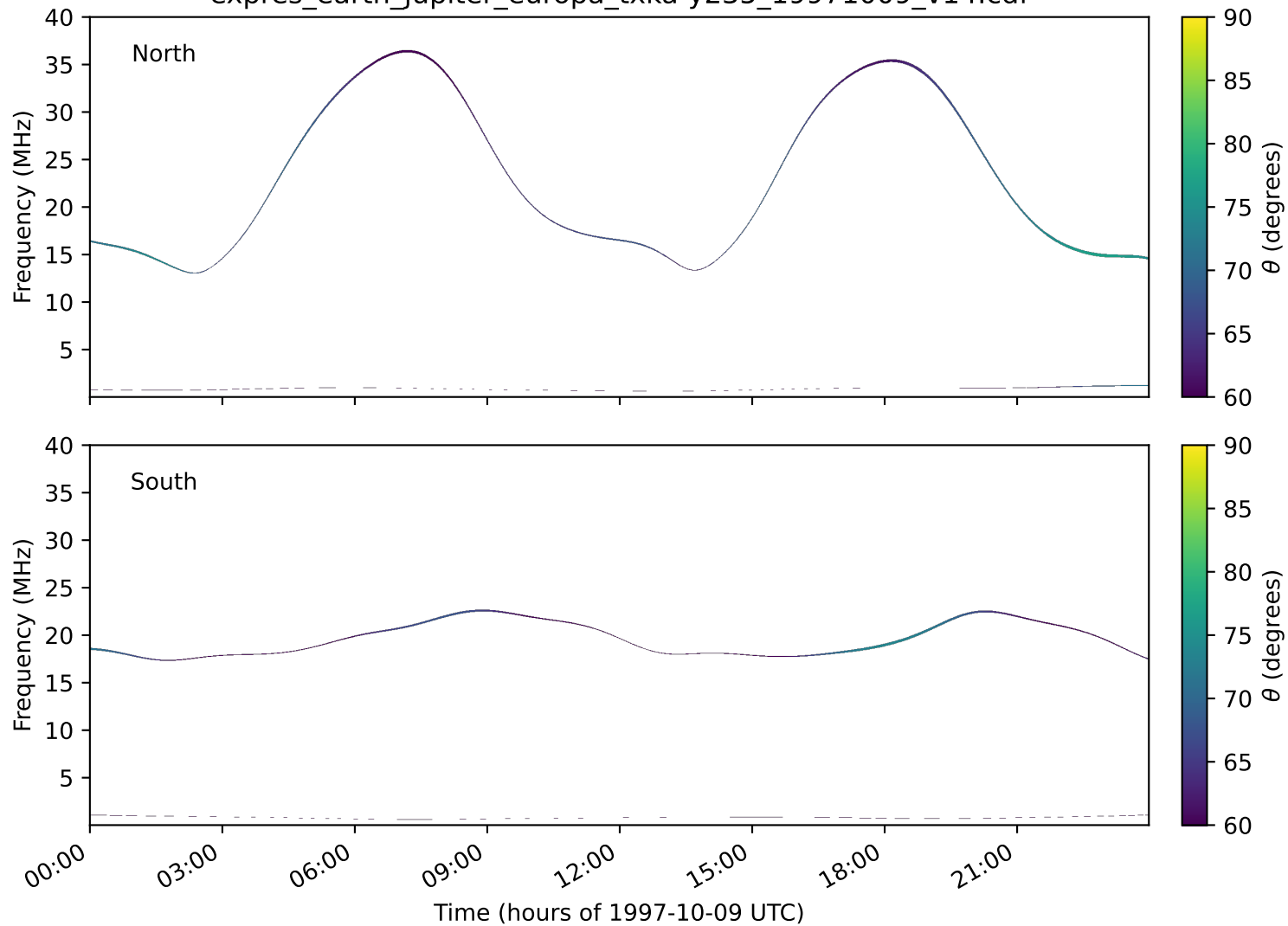
expres_earth_jupiter_europa_txka-y235_19971009_v14.cdf
