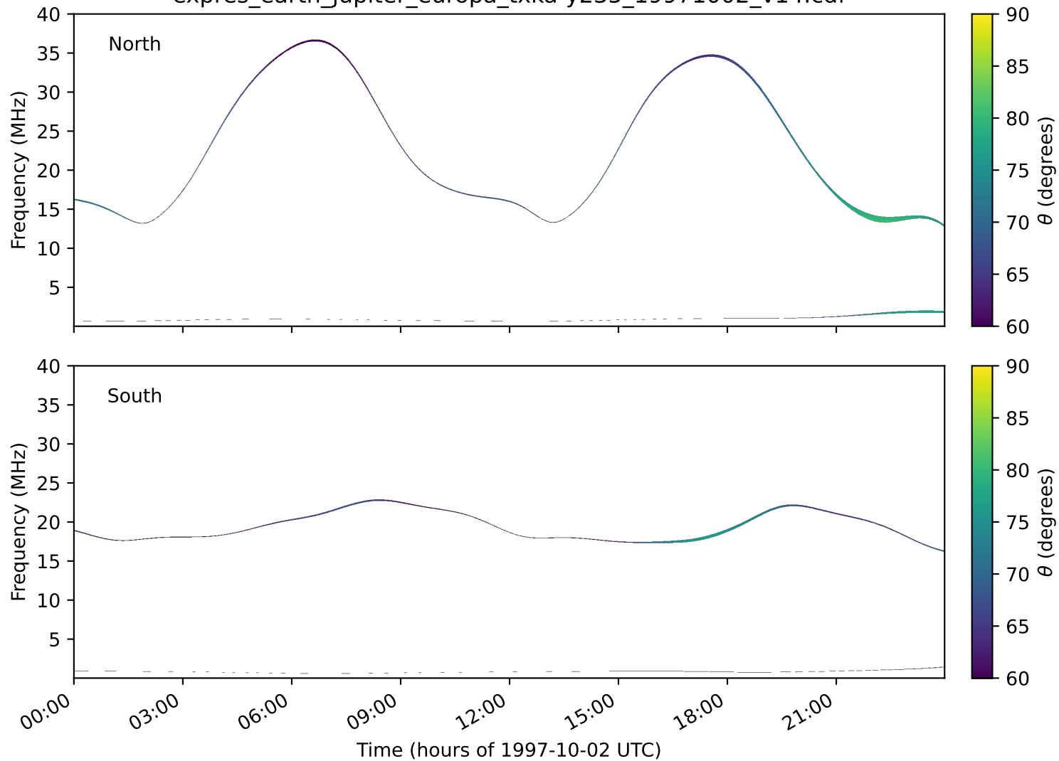
expres_earth_jupiter_europa_txka-y235_19971002_v14.cdf
