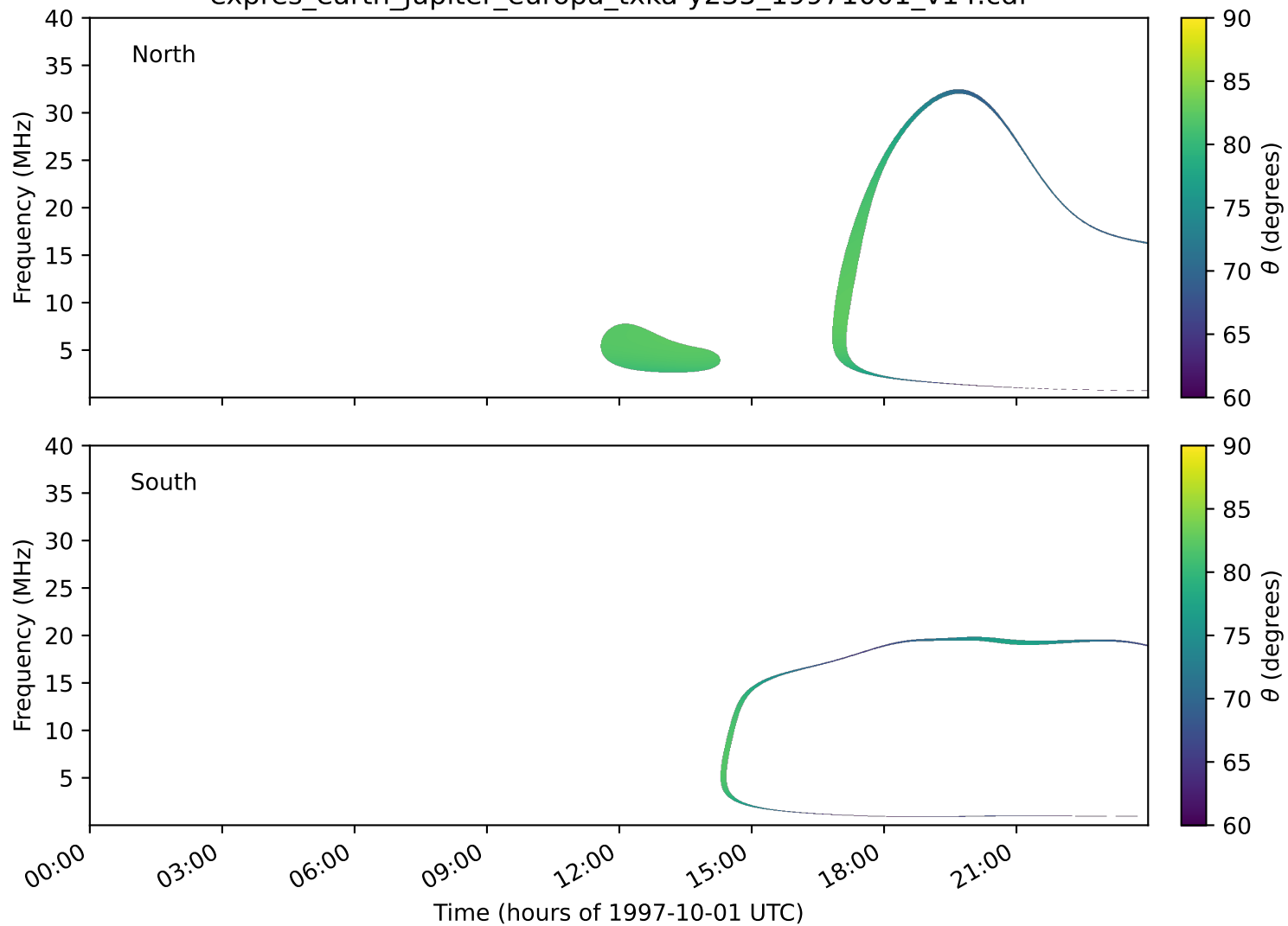
expres_earth_jupiter_europa_txka-y235_19971001_v14.cdf
