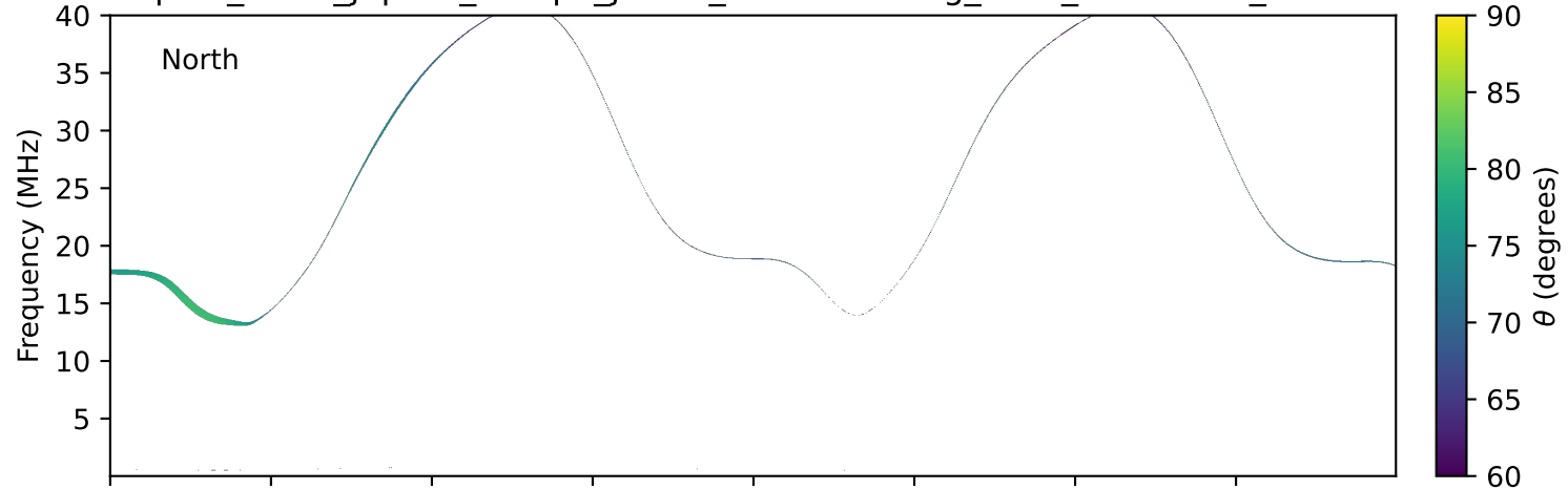
expres_earth_jupiter_europa_jrm33_lossc-wid1deg_3kev_19971016_v11.cdf
