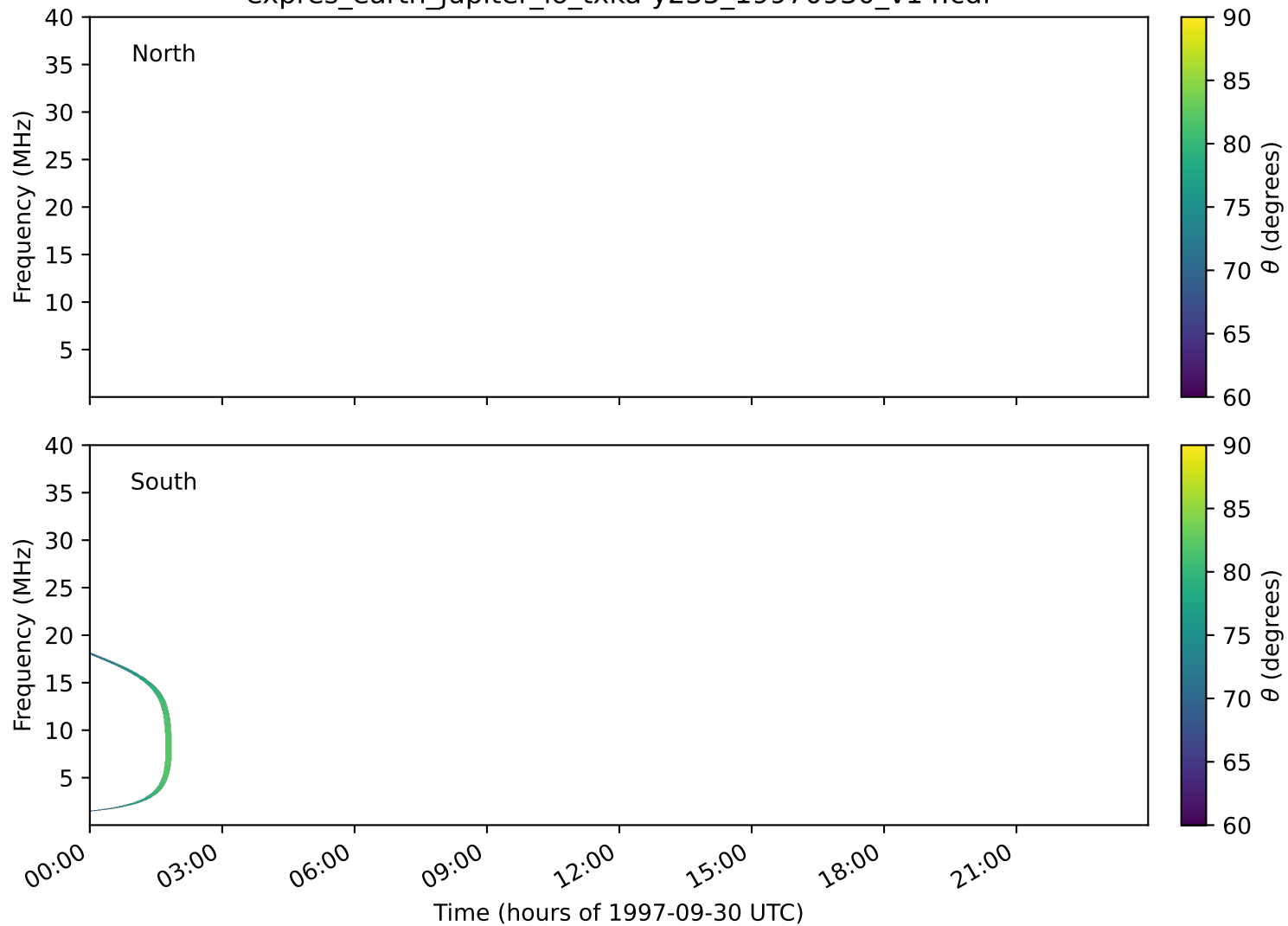
expres_earth_jupiter_io_txka-y235_19970930_v14.cdf
