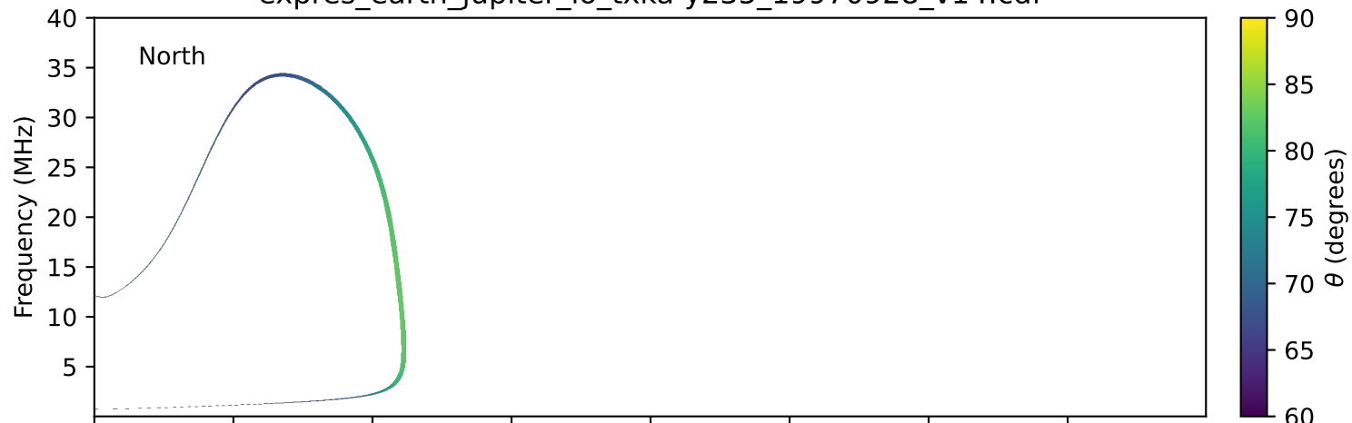
expres_earth_jupiter_io_txka-y235_19970928_v14.cdf
