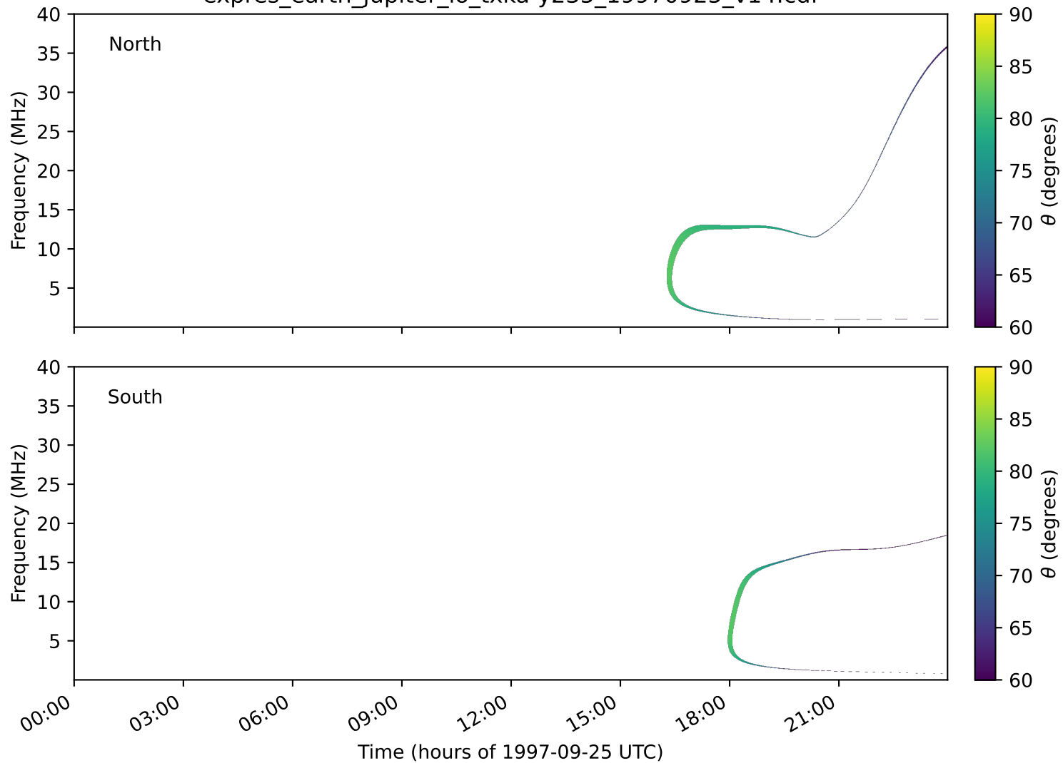
expres_earth_jupiter_io_txka-y235_19970925_v14.cdf
