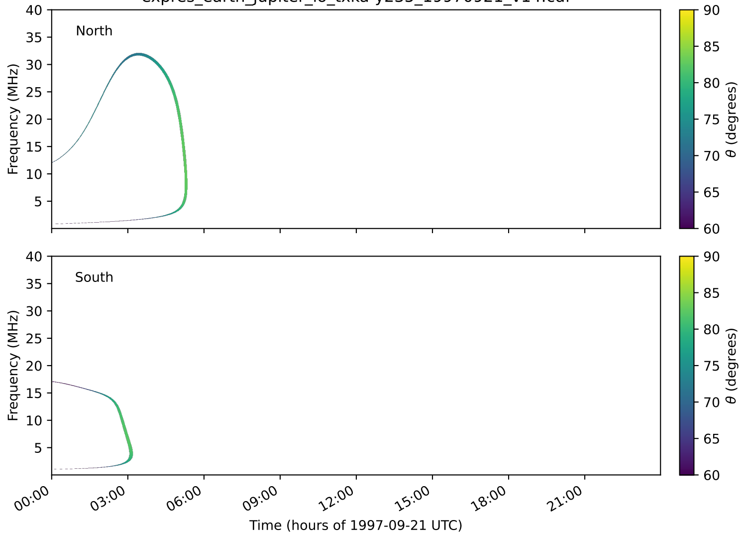
expres_earth_jupiter_io_txka-y235_19970921_v14.cdf
