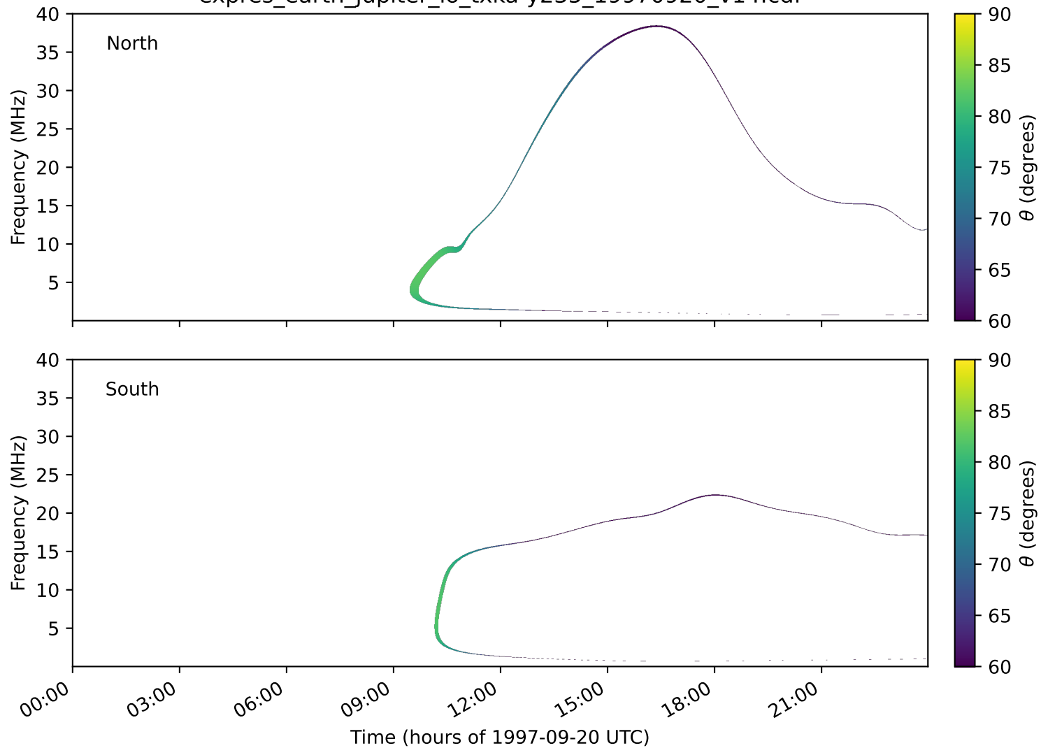
expres_earth_jupiter_io_txka-y235_19970920_v14.cdf
