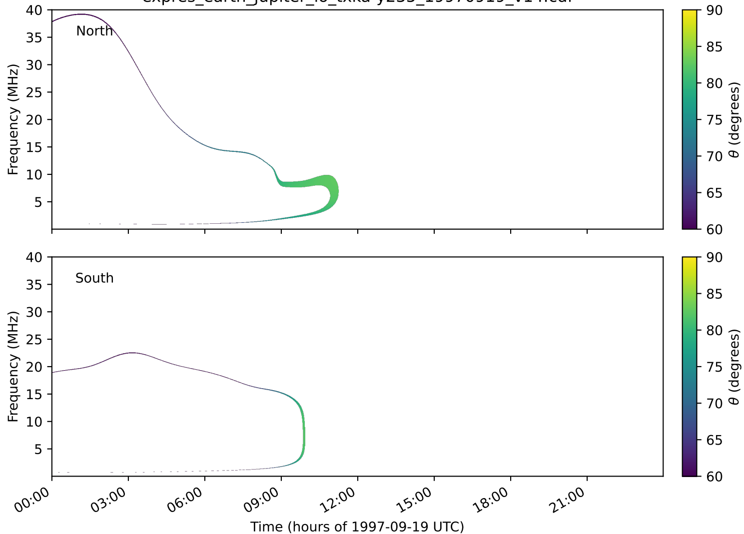
expres_earth_jupiter_io_txka-y235_19970919_v14.cdf
