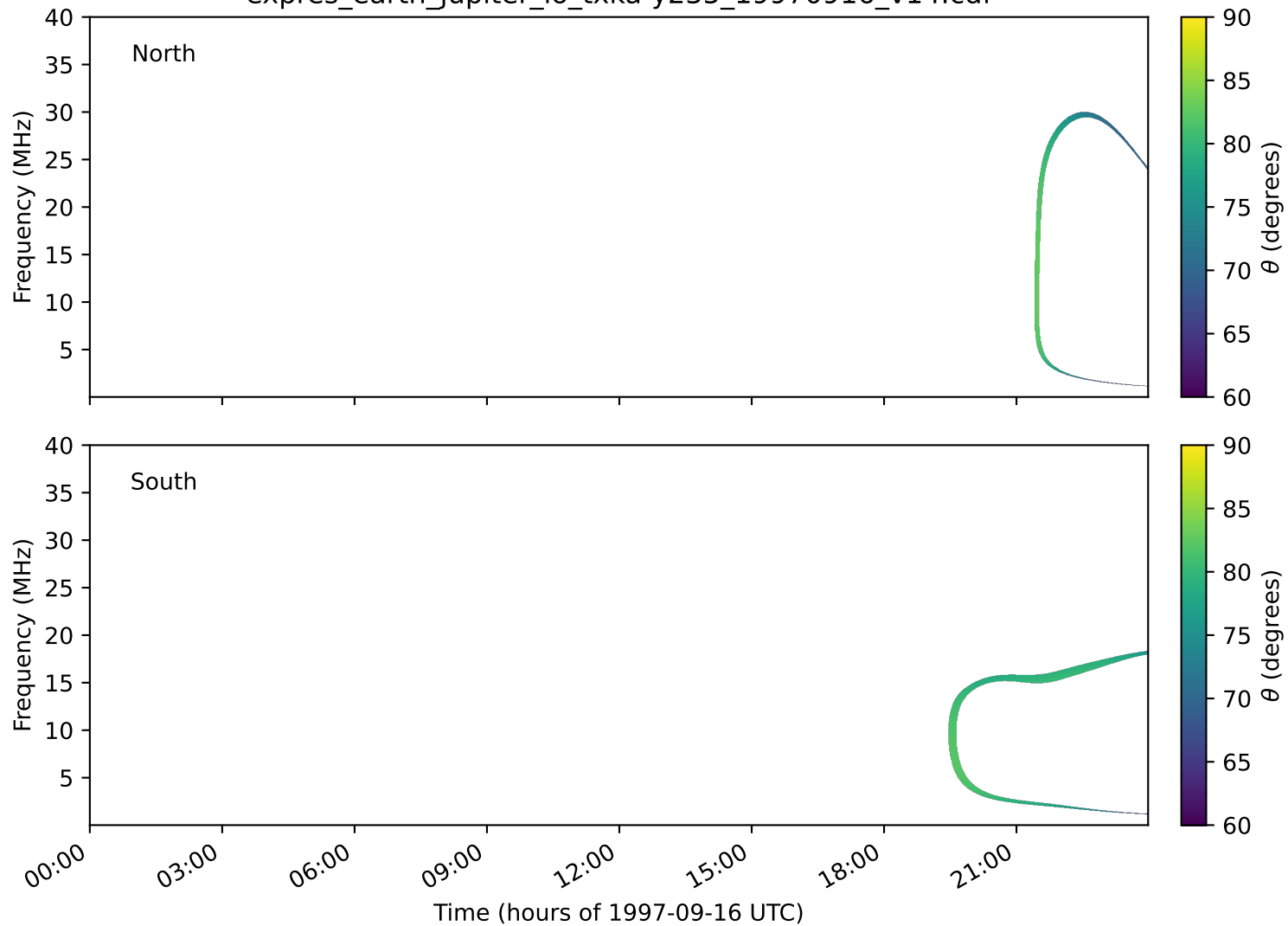
expres_earth_jupiter_io_txka-y235_19970916_v14.cdf
