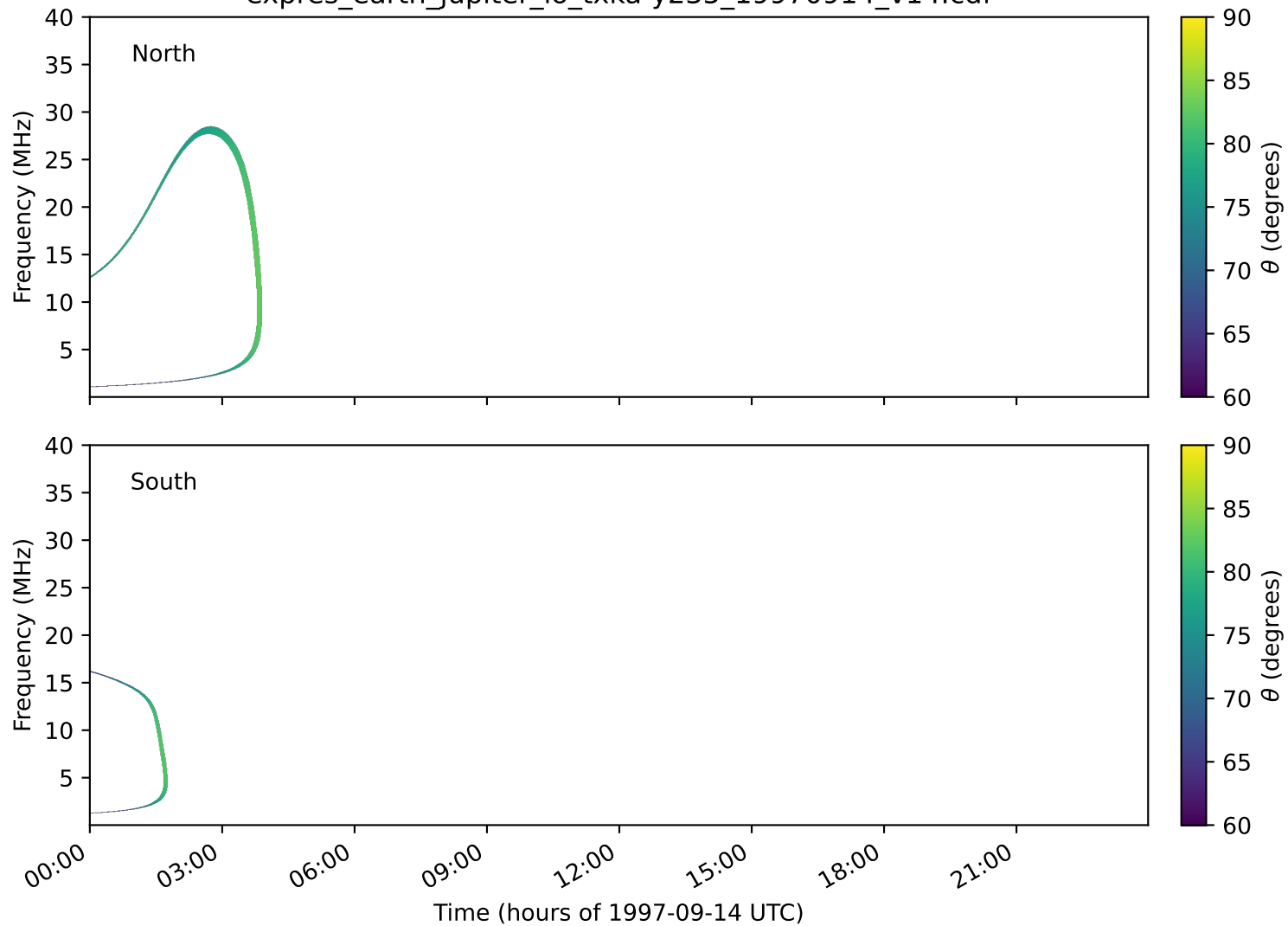
expres_earth_jupiter_io_txka-y235_19970914_v14.cdf
