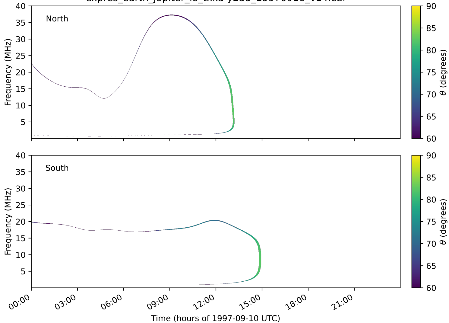
expres_earth_jupiter_io_txka-y235_19970910_v14.cdf
