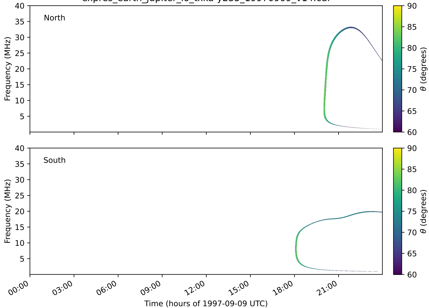
expres_earth_jupiter_io_txka-y235_19970909_v14.cdf
