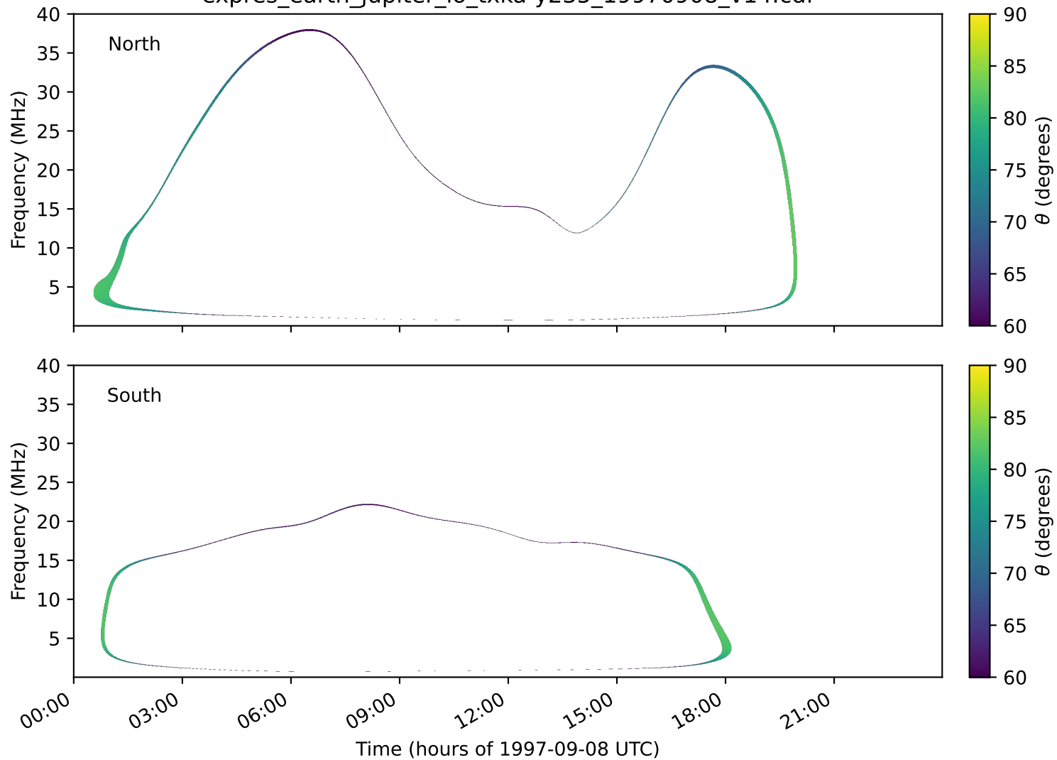
expres_earth_jupiter_io_txka-y235_19970908_v14.cdf
