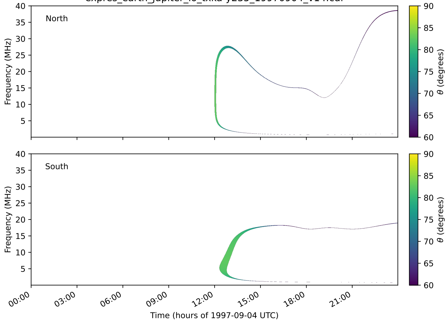
expres_earth_jupiter_io_txka-y235_19970904_v14.cdf
