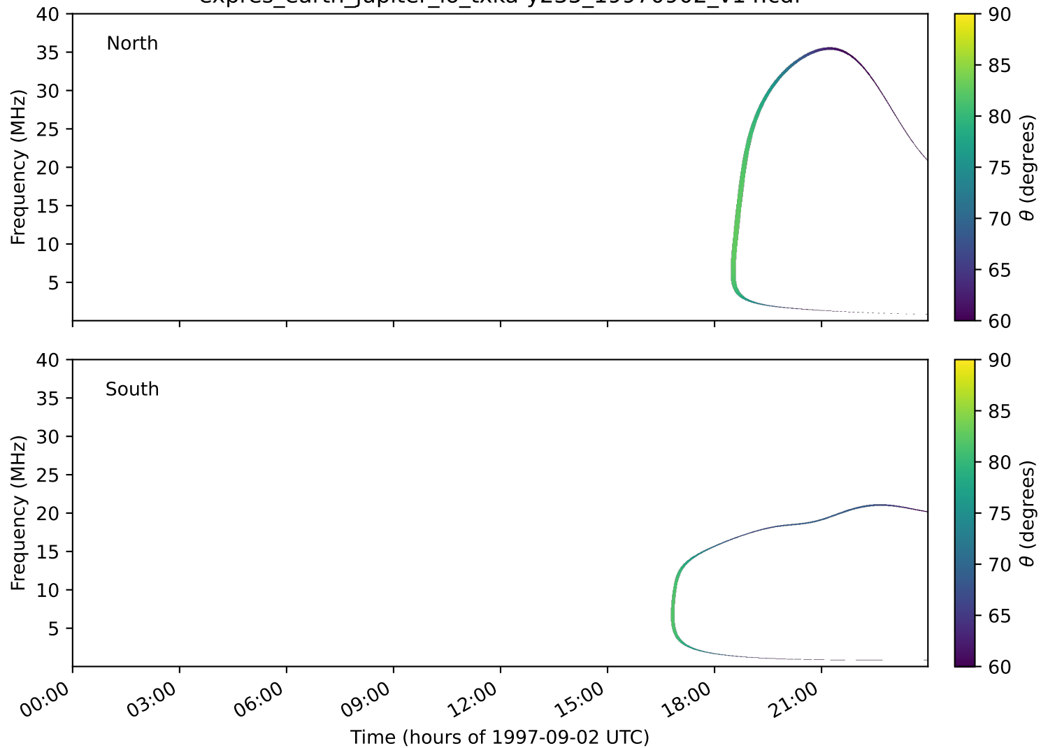
expres_earth_jupiter_io_txka-y235_19970902_v14.cdf
