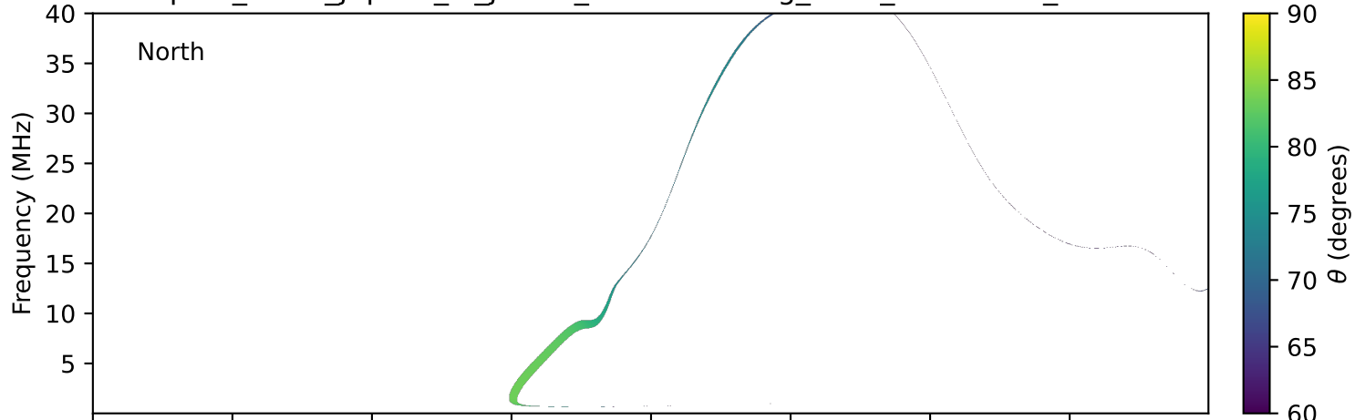
expres_earth_jupiter_io_jrm33_lossc-wid1deg_3kev_19970920_v11.cdf
