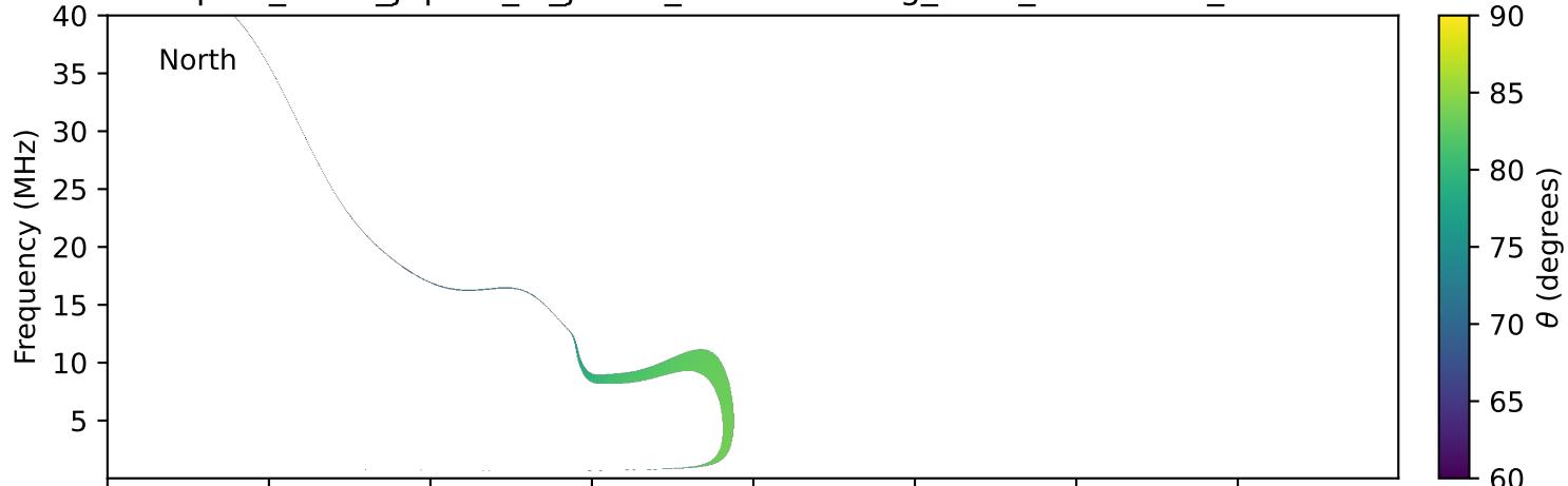
expres_earth_jupiter_io_jrm33_lossc-wid1deg_3kev_19970919_v11.cdf
