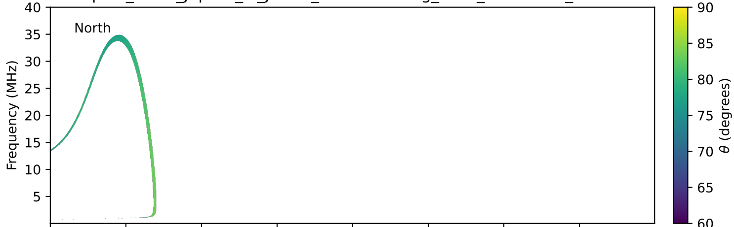
expres_earth_jupiter_io_jrm33_lossc-wid1deg_3kev_19970914_v11.cdf
