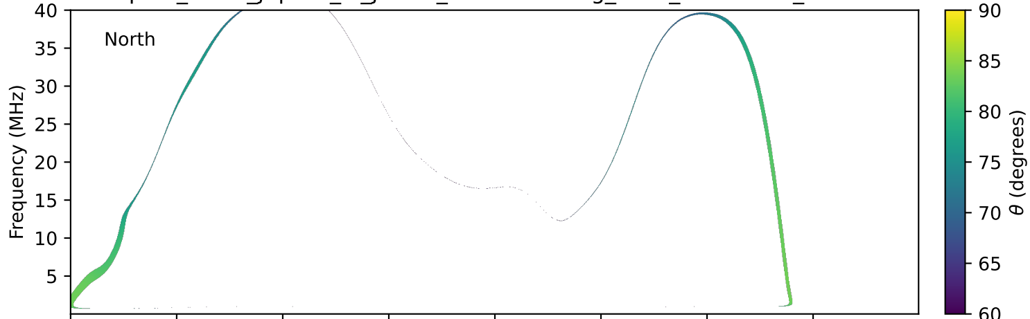
expres_earth_jupiter_io_jrm33_lossc-wid1deg_3kev_19970908_v11.cdf
