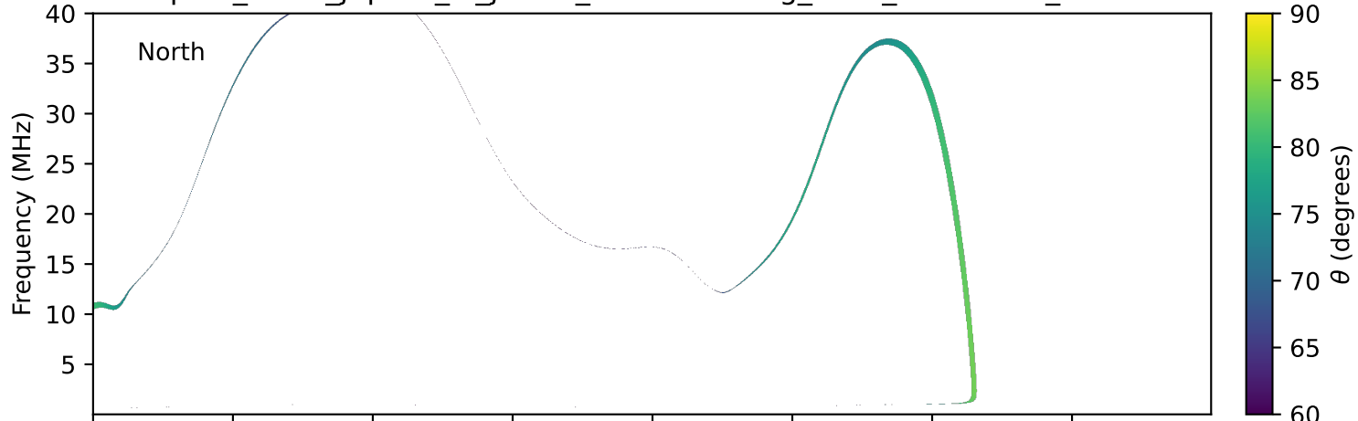
expres_earth_jupiter_io_jrm33_lossc-wid1deg_3kev_19970901_v11.cdf
