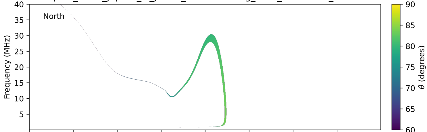
expres_earth_jupiter_io_jrm09_lossc-wid1deg_3kev_19970926_v11.cdf
