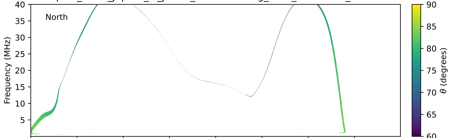
expres_earth_jupiter_io_jrm09_lossc-wid1deg_3kev_19970908_v11.cdf
