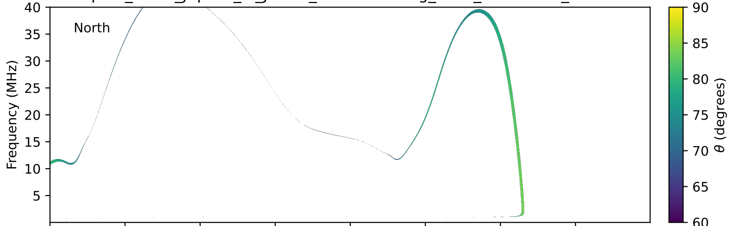
expres_earth_jupiter_io_jrm09_lossc-wid1deg_3kev_19970901_v11.cdf
