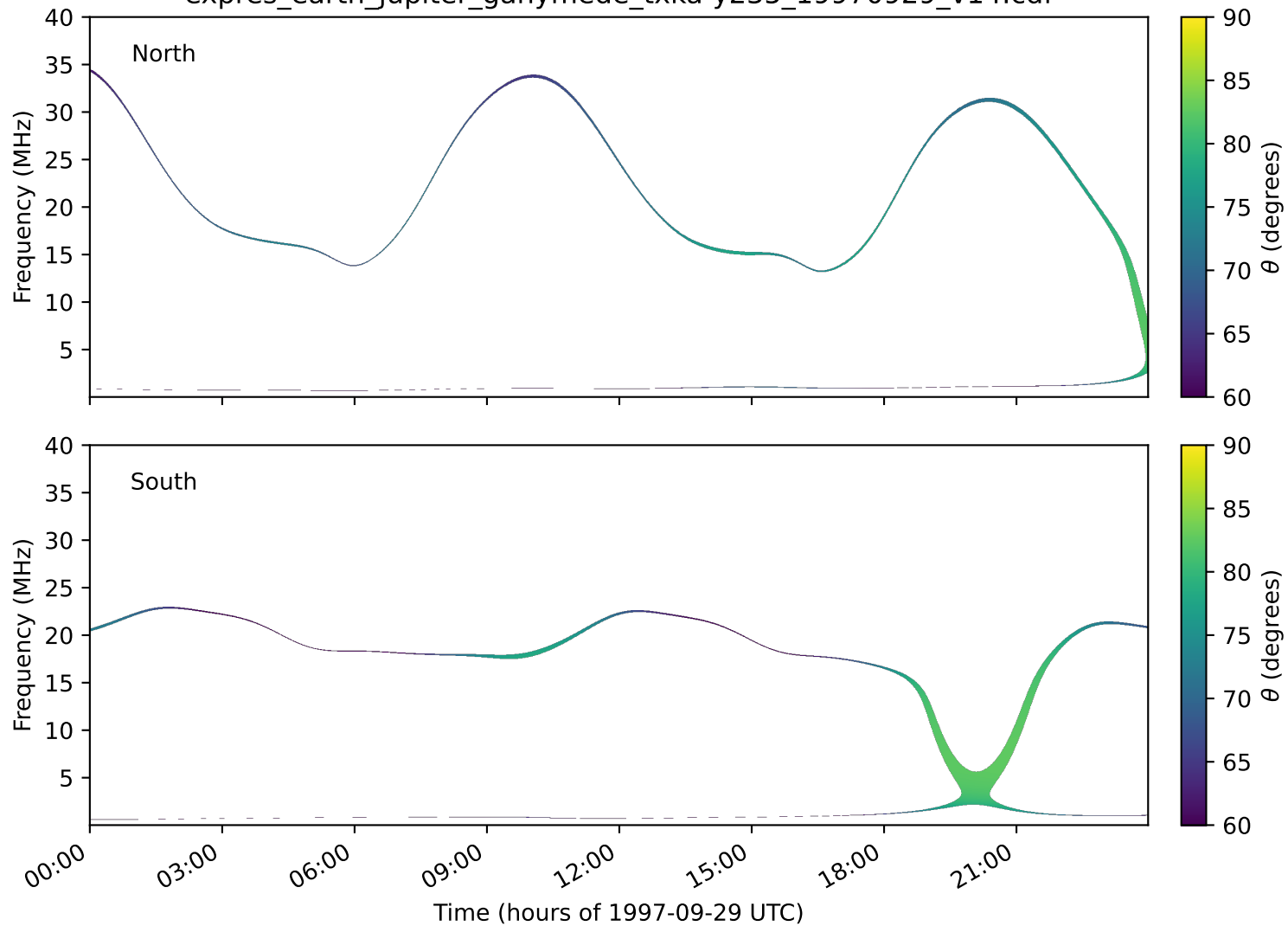
expres_earth_jupiter_ganymede_txka-y235_19970929_v14.cdf
